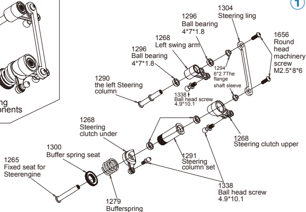
1265 Fixed seat for Steerengine
