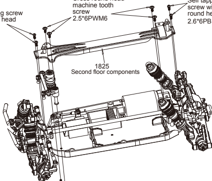
0114 Cross countersunk head screw 2.5*8KM
